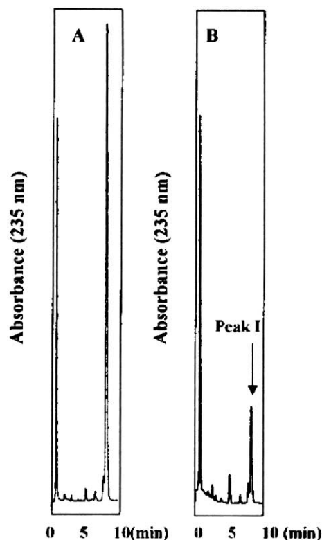
Figure 1. An example of the HPLC analysis of purified recombinant Arabidopsis AOS activity. The enzyme reaction was carried out by incubation of purified AOS (1 pmol, either heated or fresh enzyme) with 13( S )-hydroperoxylinolenic acid (2 ng) as substrate at 25 °C for 30 min. The HPLC procedure is described in the Experimental. Chromatograms shown are: A, a heated sample of AOS; B, a fresh sample of AOS. The example shown was replicated three times to establish repeatability. This system was then used to establish AOS inhibitory activity (IC 50 ) of novel compounds a–k , ketoconazole and ASA.
