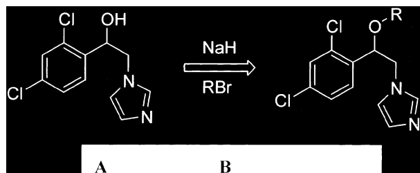
Scheme 1. Synthesis of compounds of general structure.
